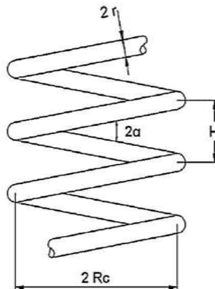
Figure : 1 Geometry of helical tube
