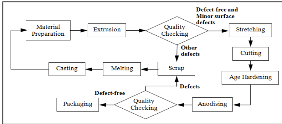
Figure 5: Improved production process of aluminium extrusion
