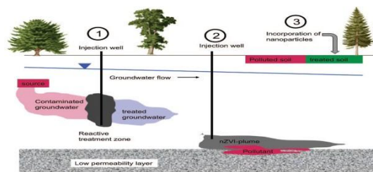
Fig 4. In situ technologies used to treat polluted groundwater and soils: (1) injection of nZVI to form a reactive barrier; (2) injection of mobile nZVI to form an nZVI plume; (3) incorporation of NP into topsoil to adsorb or degrade pollutants.
