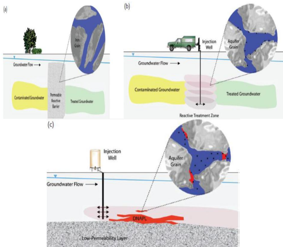
Fig.3- Three approaches to application of Fe particles for ground water remediation:
