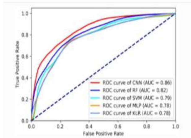
Fig. 2 Accuracy Graph
