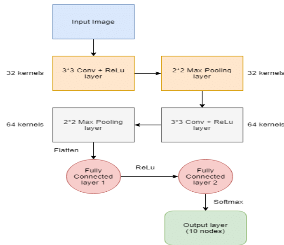
Fig. 1 Architecture
