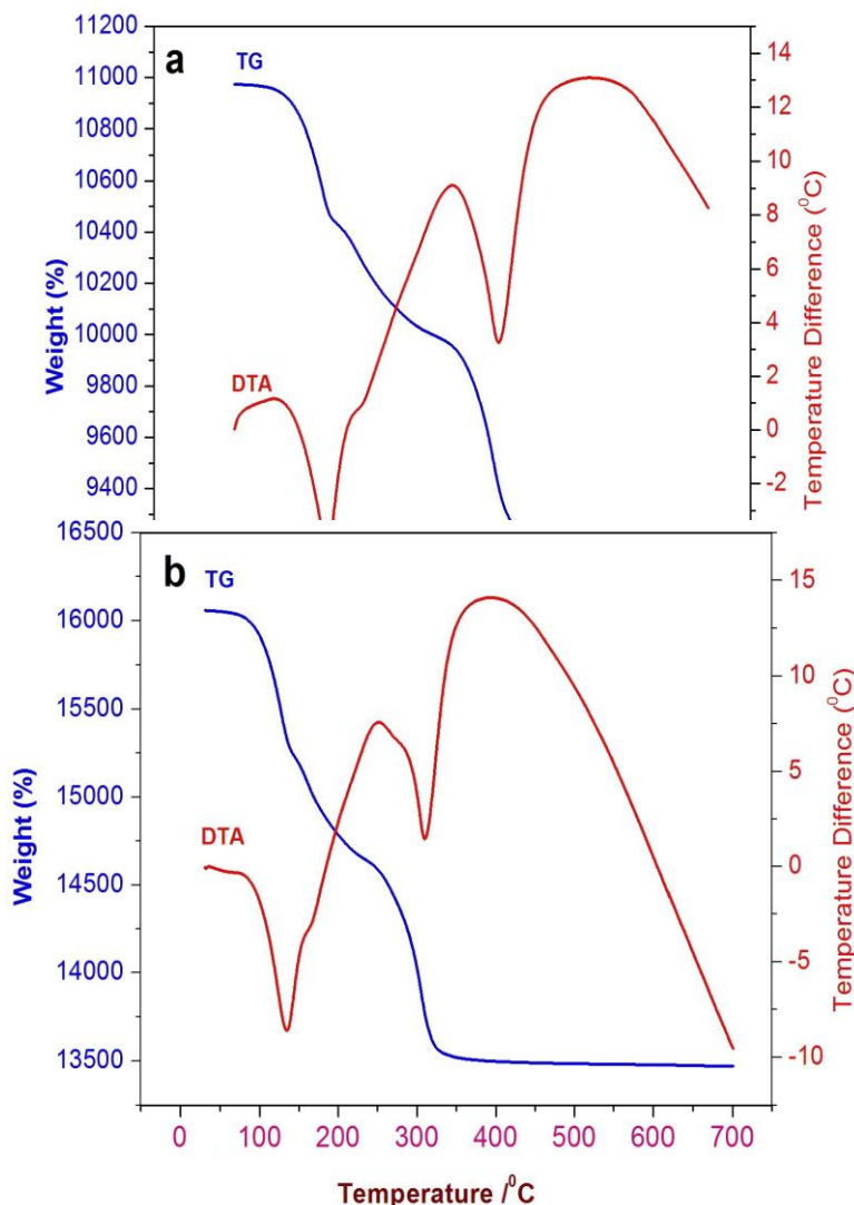
Fig.6. showing recording of TG curves for (a) phosphate Magnesium hydrogen (MZHP).
