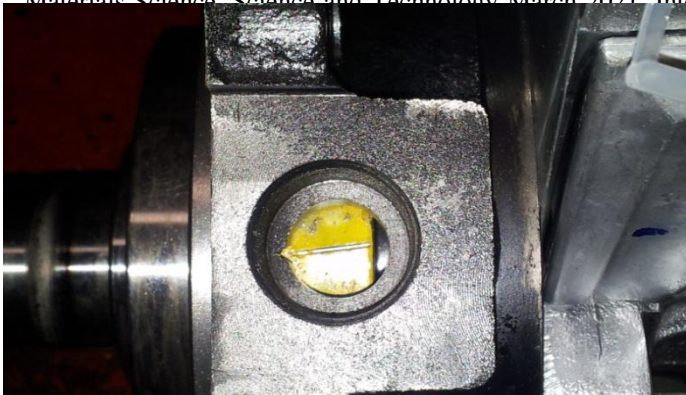
Fig. 10 Wrong Injection Timing
