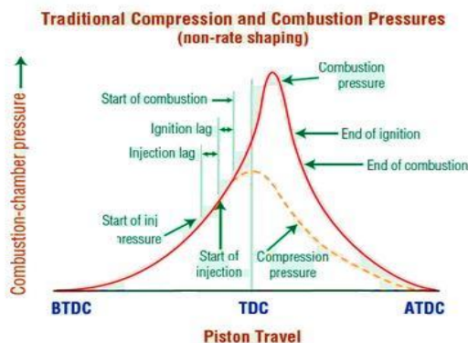
Fig 2 - Injection timing
