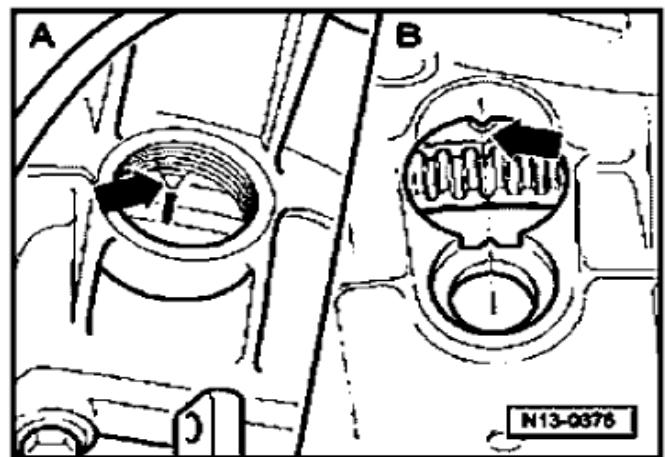
Fig:15 Injection Timing Setting in FIP & Flywheel (a) - FIP, (b) - Flywheel
