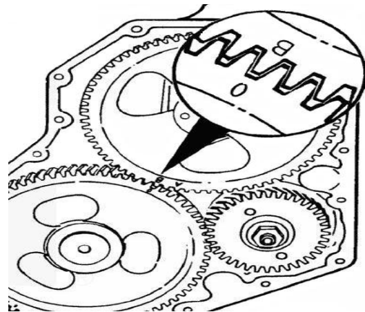
Fig 3 – Valve Timing Gears
