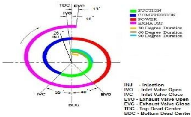
Fig 1 - Valve timing for 4 stroke CI engine
