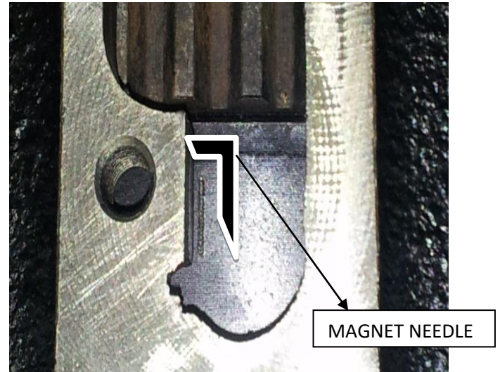
FIG:9 Timing Mark in flywheel.
