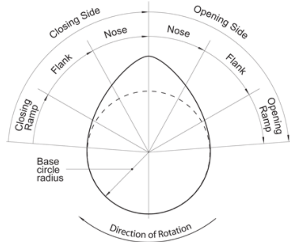
Fig.4 THE CAM LOBE
