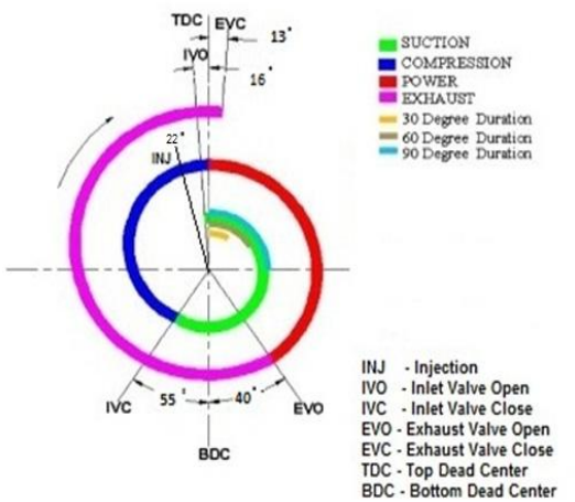
Fig.8 – Wrong Valve Timing for 4 Stroke CI engine
