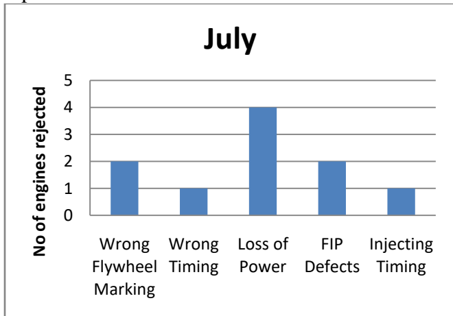
Graph. 4 - Engine Rejection Rate in July
