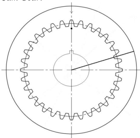
Fig.5 -Cam gear
