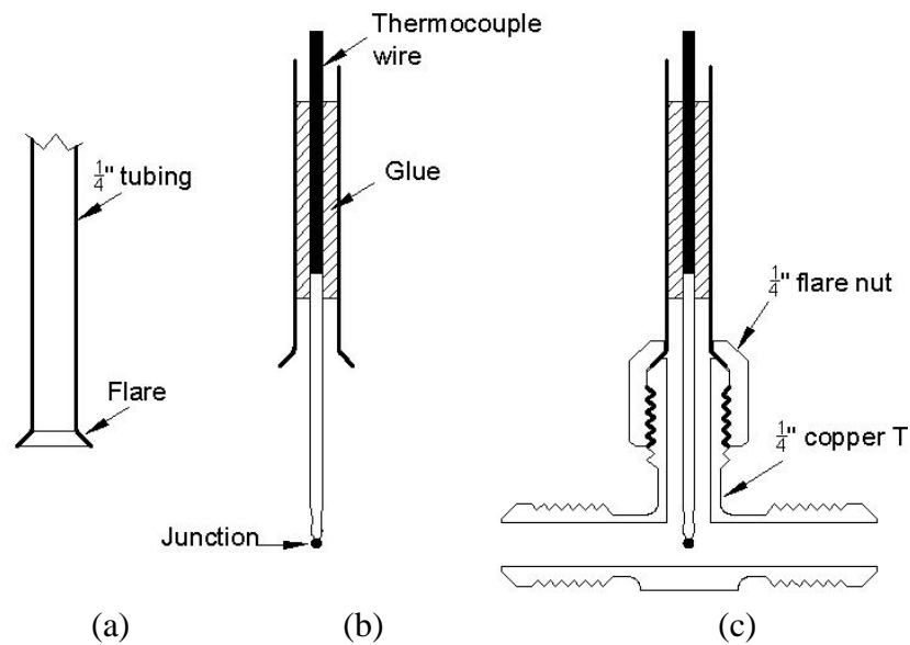
Figure 3: Construction method of temperature measurement point
