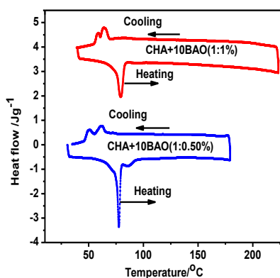
FIGURE 2. DSC thermogram of C and D HBLC complex.
