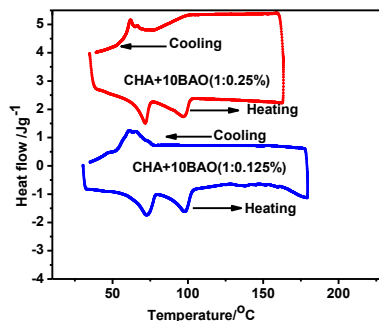
. FIGURE 1. DSC thermogram of A and B HBLC Complex
