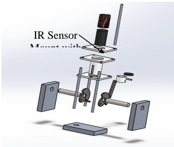
Figure 2 Assemble parts of engine
