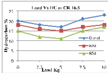
Figure: 7 Variation of Unburned HC with Loads
